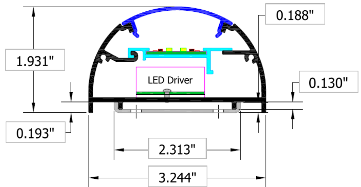
Surface Mount
