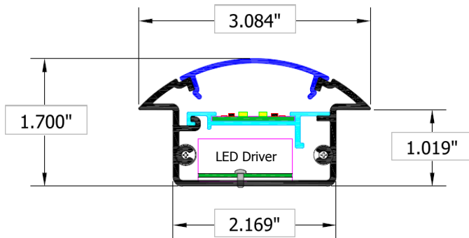
Flush Mount
